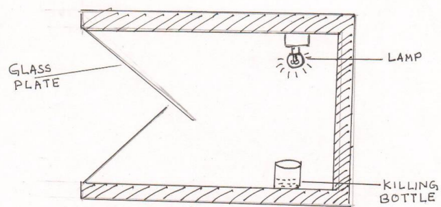
LIGHT TRAP
